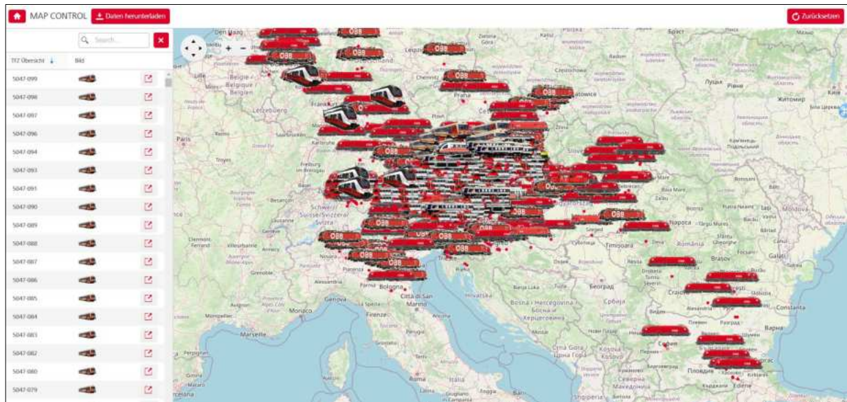
Abbildung 18 – railpower MapControl
